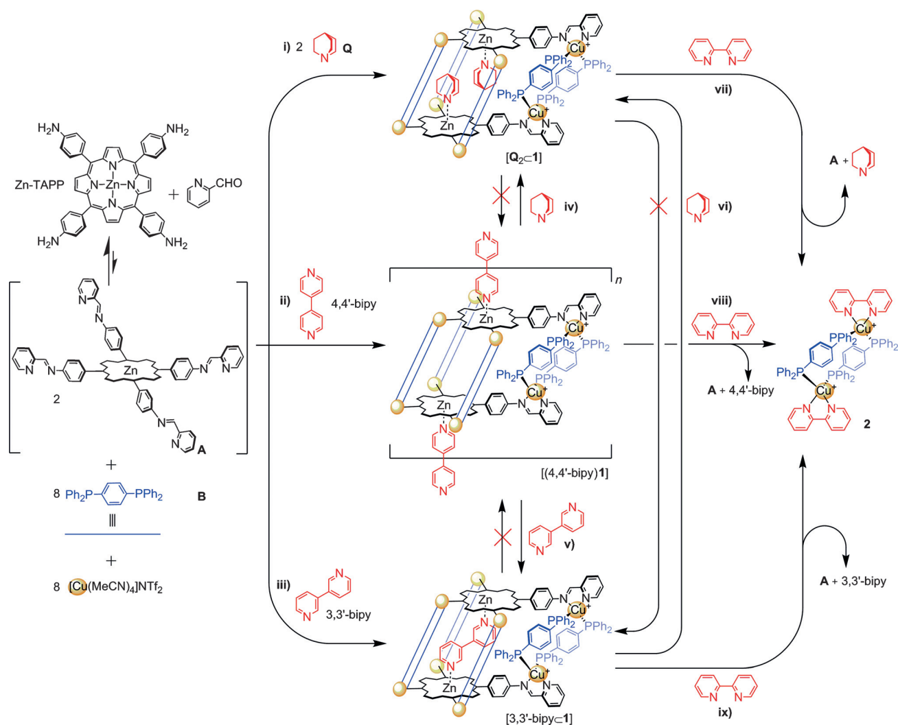
Scheme 1. Self-assembly of C_4 -symmetric tetrakis(bidentate) ligand A , 2-formylpyridine, 1,4-bis(diphenylphosphino)benzene B , and [Cu(MeCN)_4]NTf_2 with quinuclidine ( Q ) and the three bipyridine isomers (2,2', 3,3', and 4,4') in DMF to form prisms i ) [Q_2C1] (77%), ii ) [(4,4'-bipy)1] (60%), and iii ) [3,3'-bipyC1] (64%). Transformations between these complexes are also shown (iv–ix), which were monitored by ^1H NMR spectroscopy (Supporting Information, Section 4). The blue lines and orange spheres represent 1,4-bis(diphenylphosphino)benzene and Cu I , respectively.
